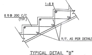
TYPICAL DETAIL "B"
