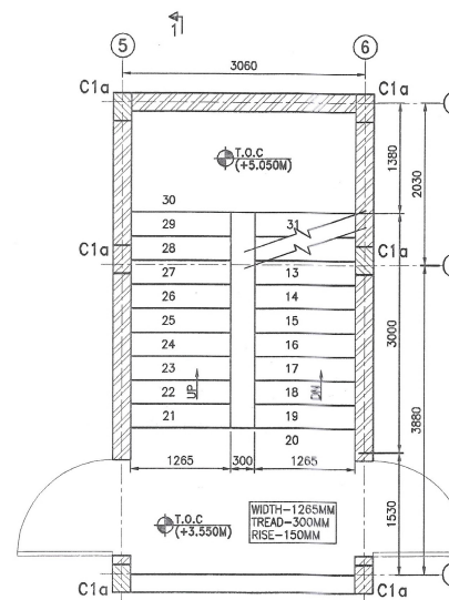
FIRST FLOOR PLAN-STAIRCASE AREA (SCALE 1:50)
