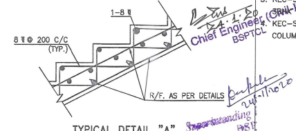
TYPICAL DETAIL "A"
