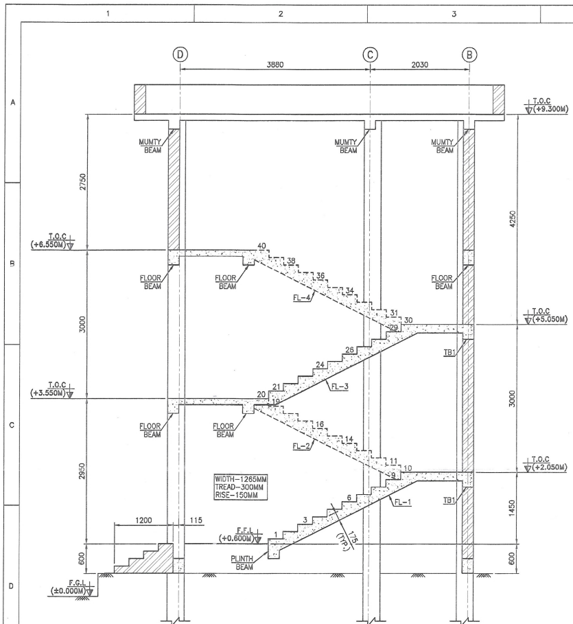
SECTION 1-1 (SCALE 1:50)
