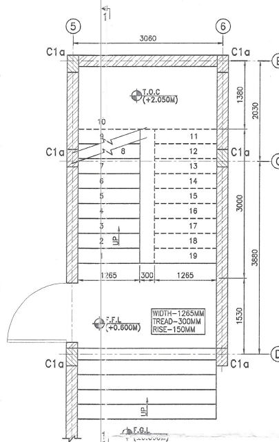
GROUND FLOOR PLAN-STAIRCASE AREA (SCALE 1:50)
