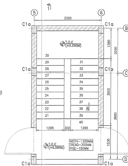
TERRACE FLOOR PLAN-STAIRCASE AREA (SCALE 1:50)
